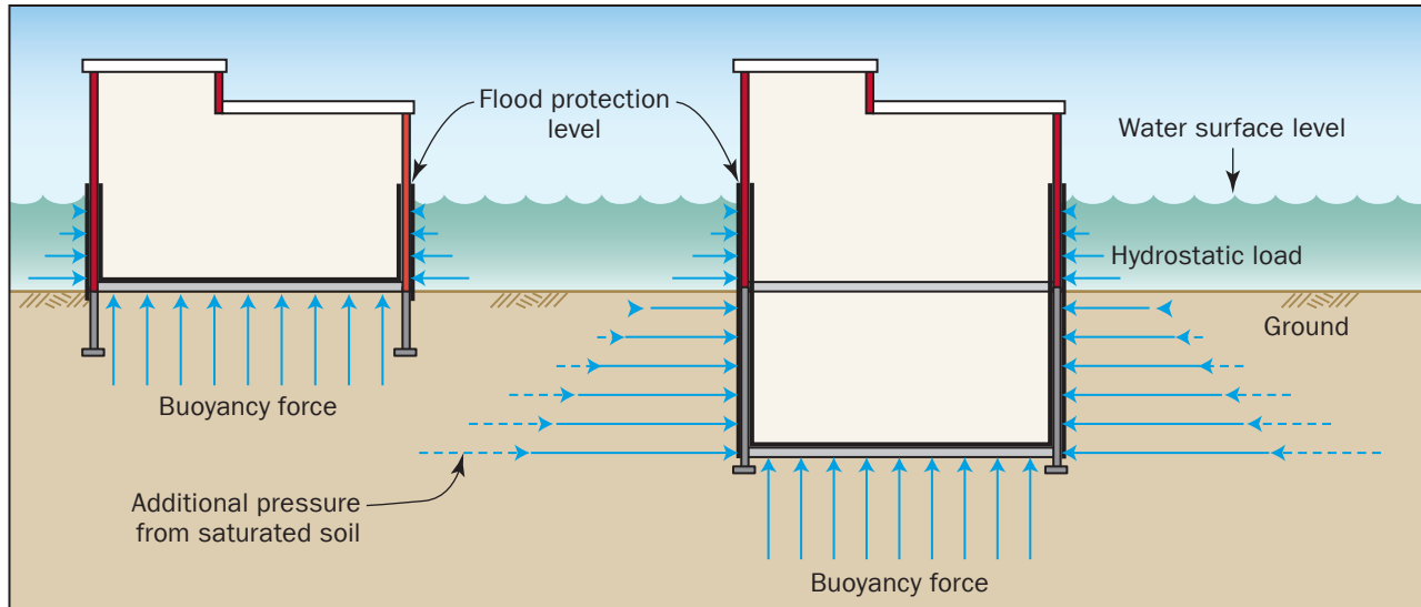
Figure 1: Hydrostatic loads
